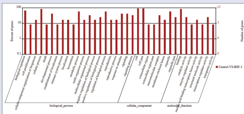
Figure 11: Gene ontology functional classification of the differentially expressed genes
