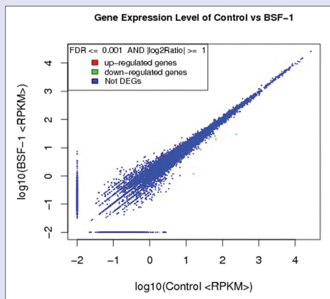
Figure 10: Scatter plot of differential expression
