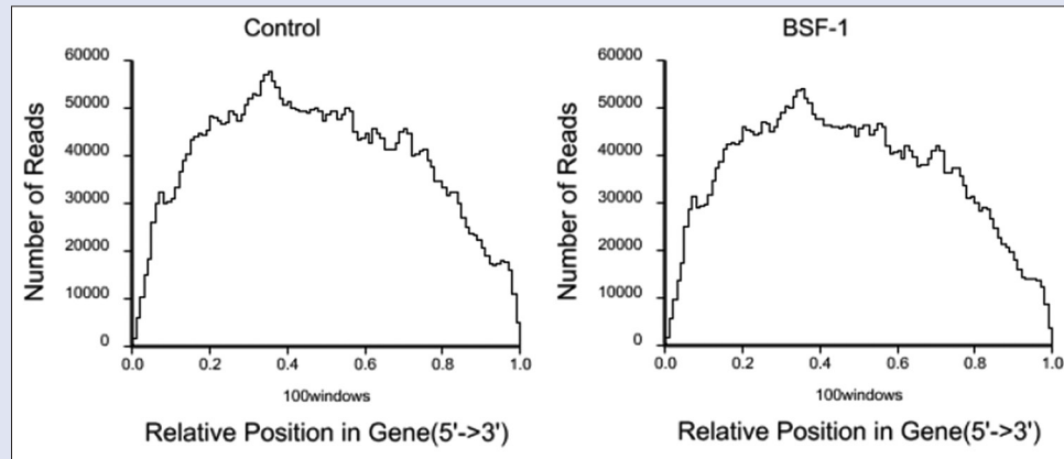
Figure 8: Randomness assessment
